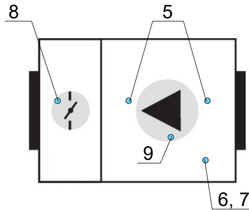
AHU overview with control and measuring equipment
