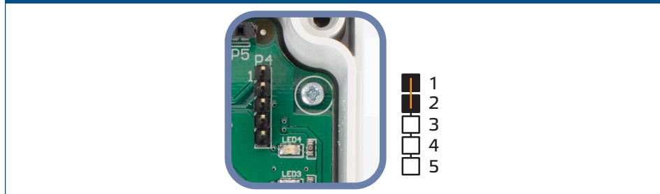
Fig. 8 Modbus holding register reset jumper
