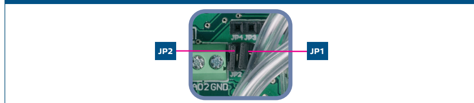
Fig. 5 Pull-up weerstand jumper
