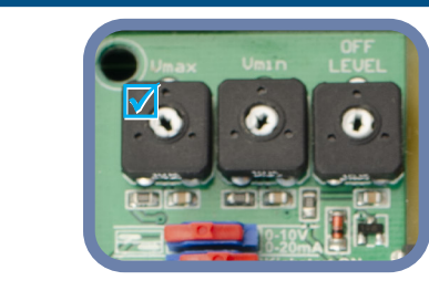
Fig. 5 Max. speed trimmer
