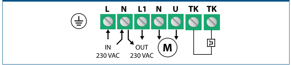
Fig. 3 Wiring and connections
