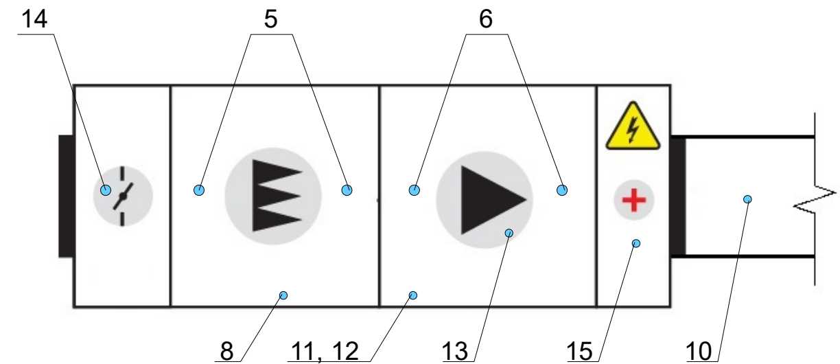
AHU overview with control and measuring equipment
